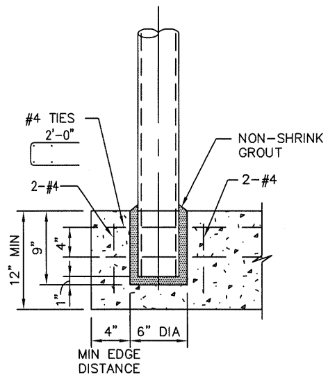
EMBEDDED GUARD POST
