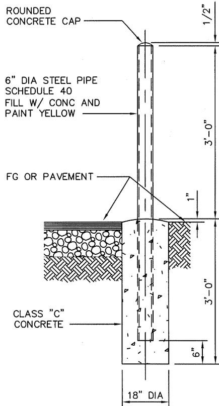
GUARD POST IN FIELD
