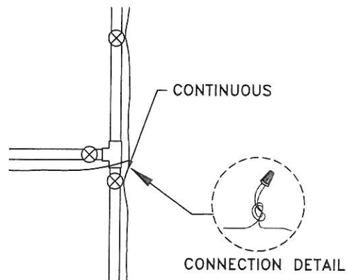
TRACER WIRE INSTALLATION DETAILS
