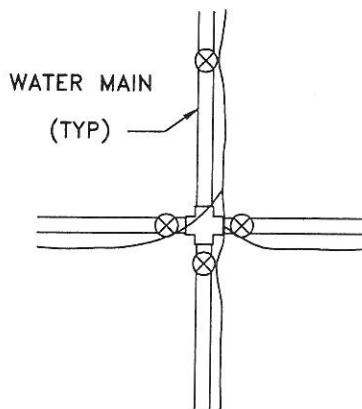
TRACER WIRE INSTALLATION DETAILS
