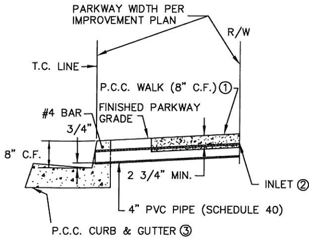
8" CURB SECTION
