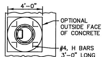
PLAN (RINGS AND COVER NOT SHOWN)
