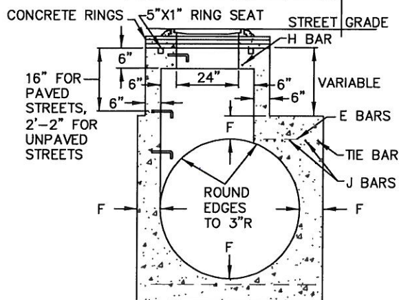
DETAIL A SEE NOTE ⑤
