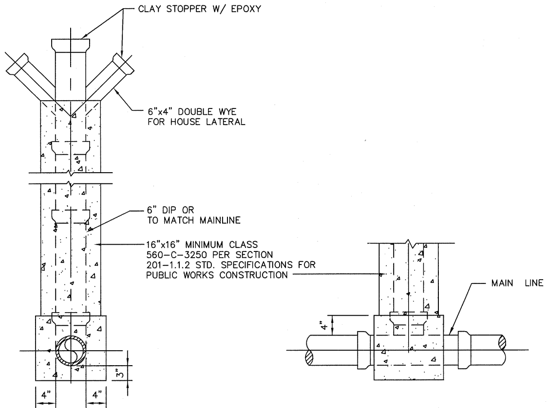
SECTION
